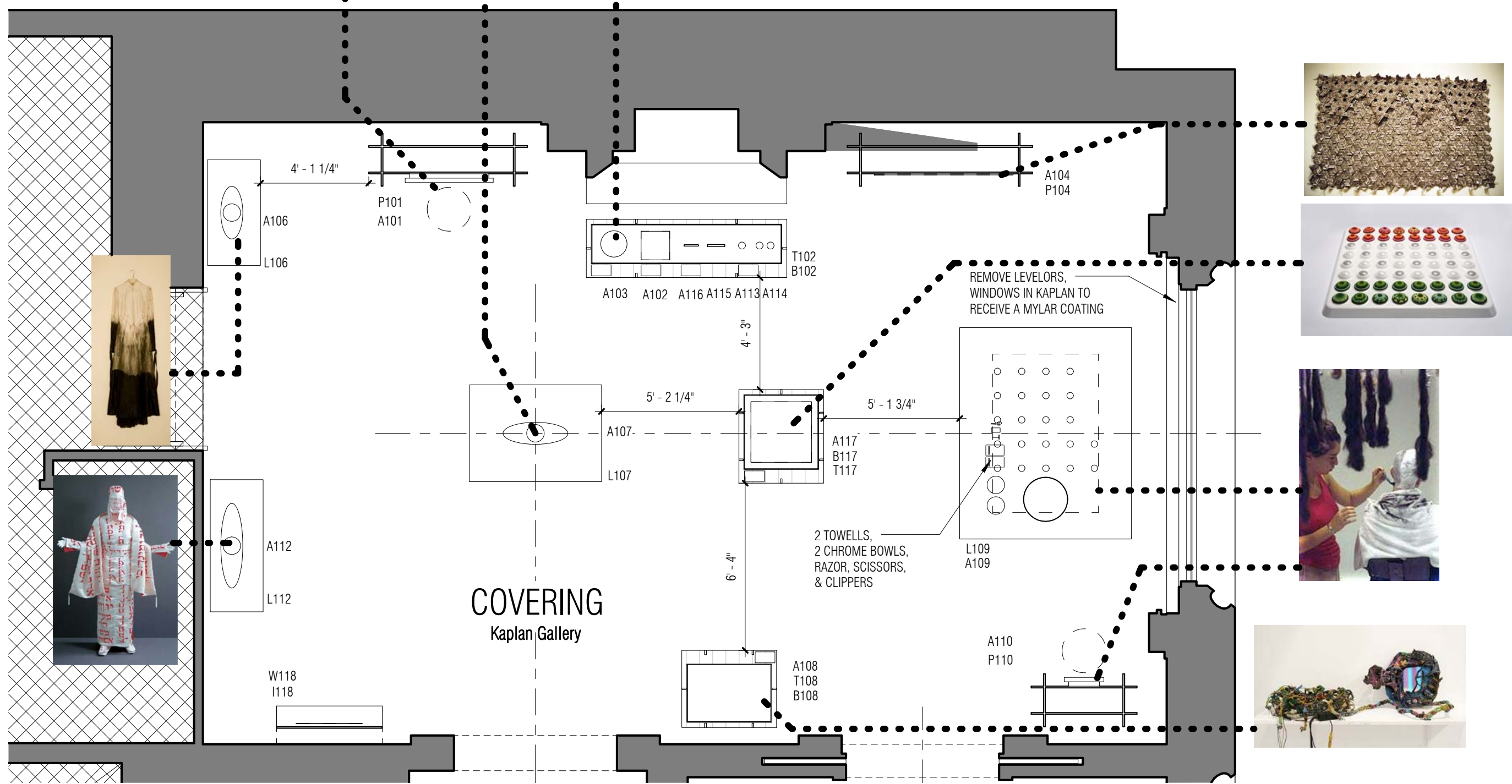
1 Kaplan Gallery 1/4" = 1'-0"
